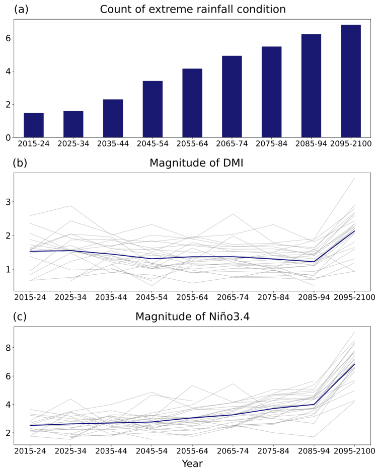
Fig. 7. The SSP5-8.5 climate change scenario: a. Frequency of concurrent conditions satisfying DMI > 0.5 and Ni\tilde{no}3.4 > 1.5 , and decadal trends of the average values of b. DMI and c. Niño3.4 index under these conditions (gray solid lines represent the results from individual models).
